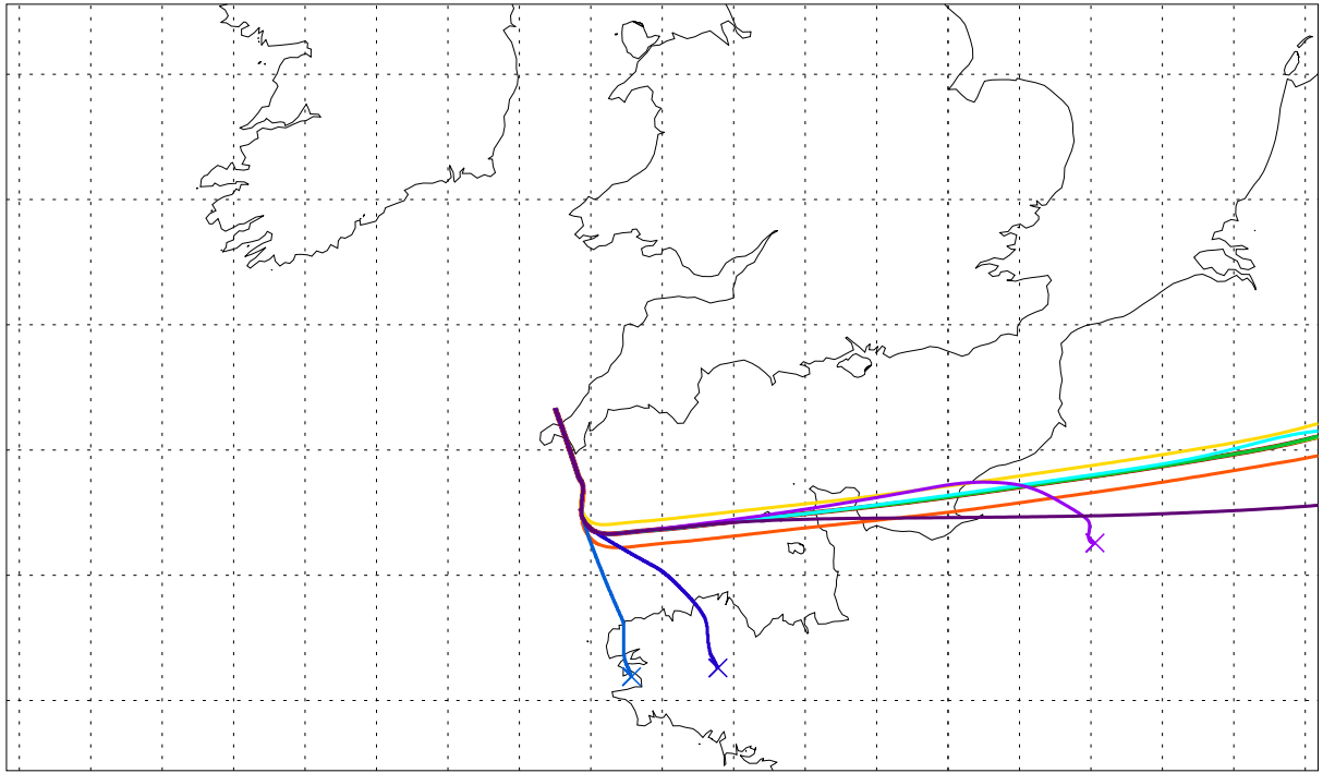
Balloon launch 12UT 24/10/2003 072hr met forecast
